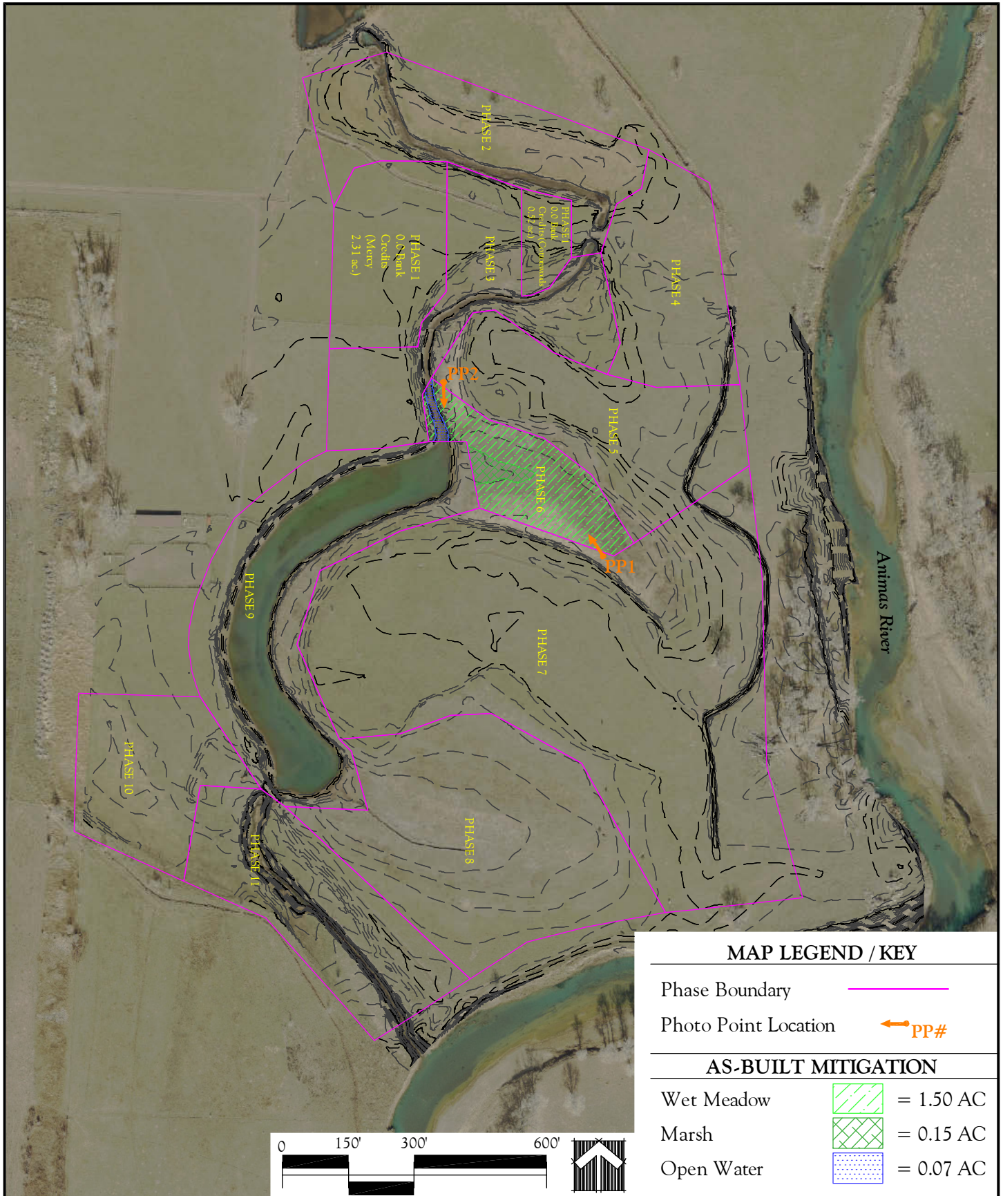
AS-BUILT PHASE 6 AS-BUILT SEPTEMBER 2010 ANIMAS RIVER WETLANDS
